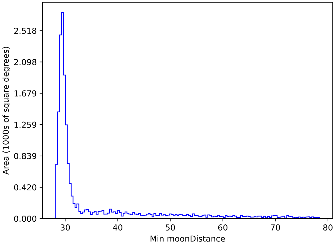
too_elab_r32_d3_griz_v3.4_10yrs WFD y band: Min moonDistance
