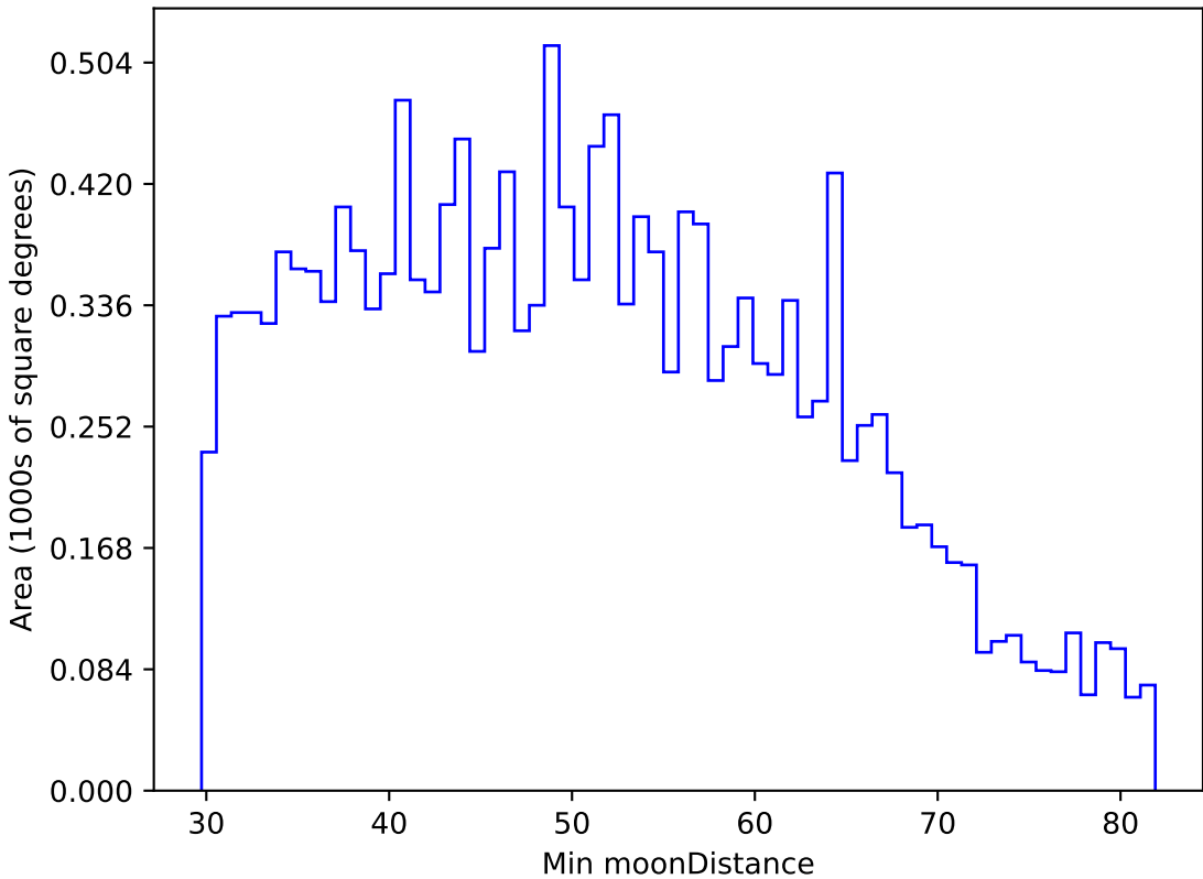
too_elab_r32_d3_griz_v3.4_10yrs WFD u band: Min moonDistance
