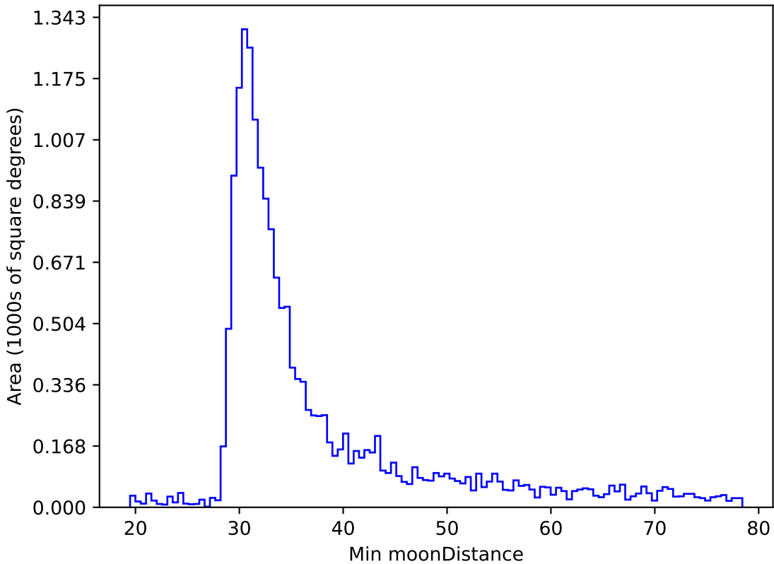
too_elab_r32_d3_griz_v3.4_10yrs WFD r band: Min moonDistance
