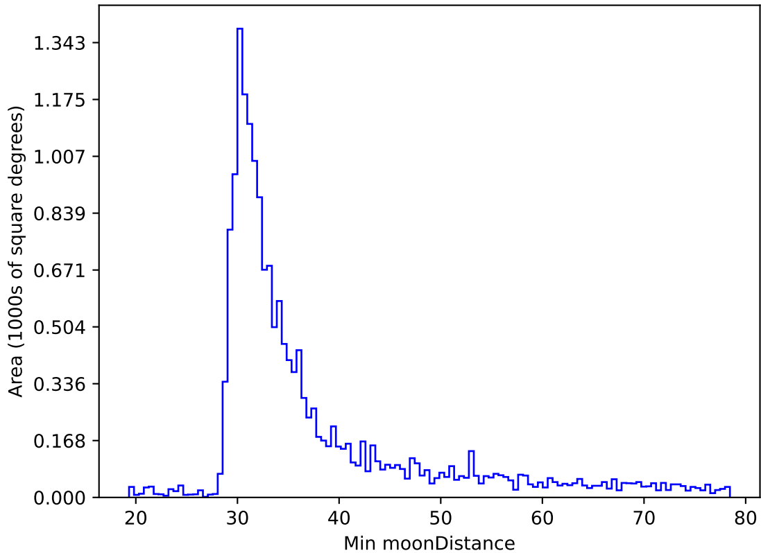
too_elab_r32_d3_griz_v3.4_10yrs WFD r band: Min moonDistance
