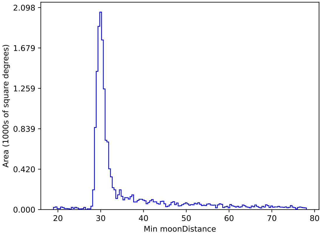
too_elab_r32_d3_griz_v3.4_10yrs WFD i band: Min moonDistance
