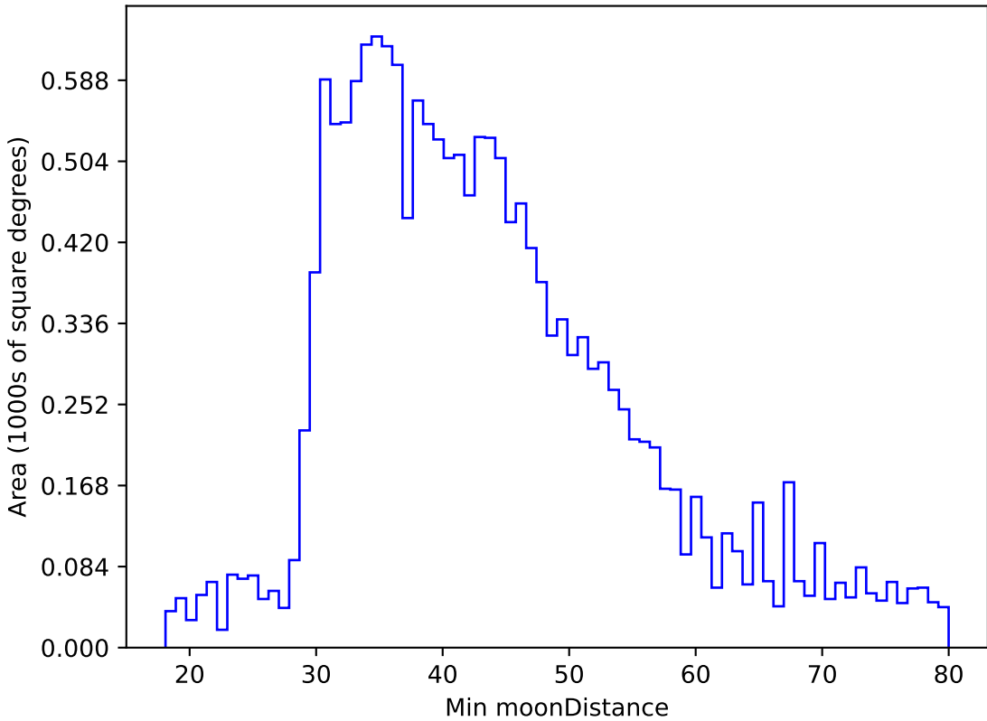
too_elab_r32_d3_griz_v3.4_10yrs WFD g band: Min moonDistance
