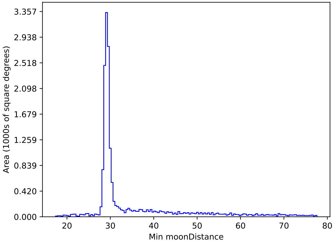
too_elab_r32_d3_griz_v3.4_10yrs WFD all bands: Min moonDistance
