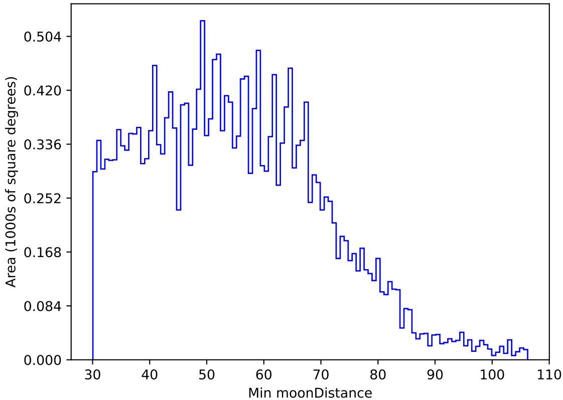
too_elab_r32_d3_griz_v3.4_10yrs All sky u band: Min moonDistance
