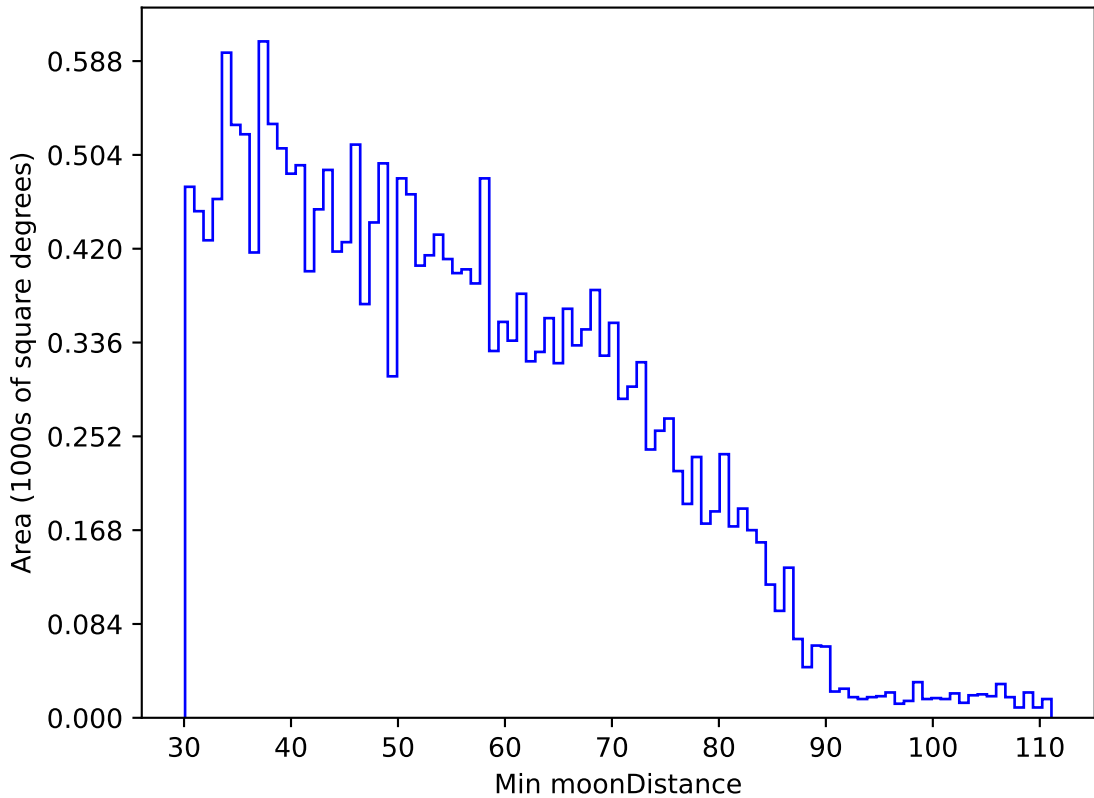
too_elab_r32_d3_griz_v3.4_10yrs All sky u band: Min moonDistance
