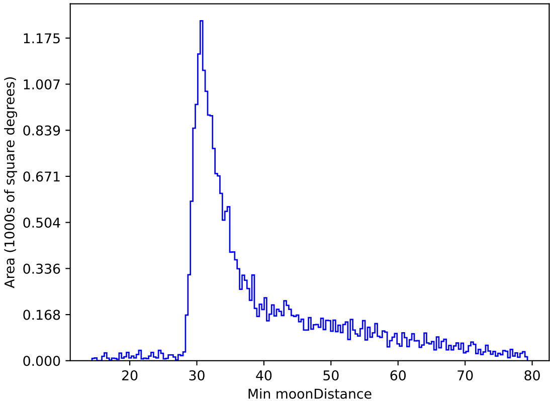
too_elab_r32_d3_griz_v3.4_10yrs All sky r band: Min moonDistance
