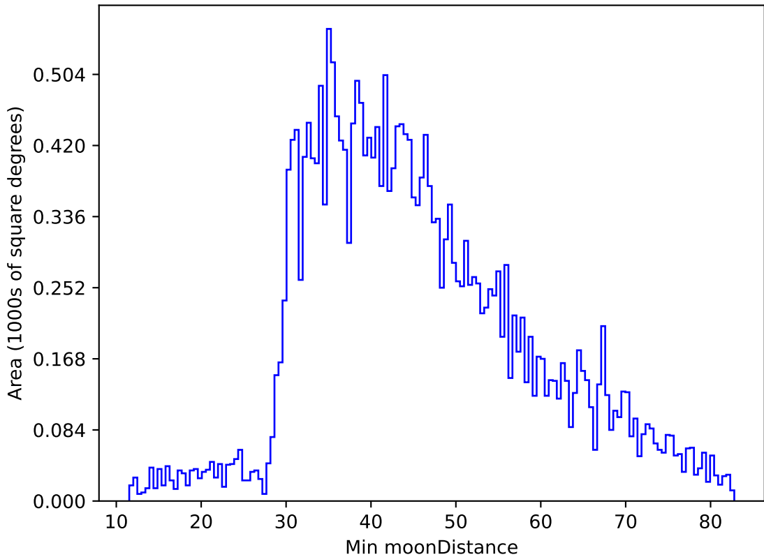
too_elab_r32_d3_griz_v3.4_10yrs All sky g band: Min moonDistance
