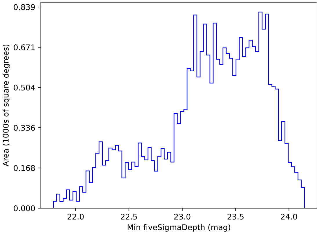
too_elab_r32_d3_griz_v3.4_10yrs Yr 1 r band: Min fiveSigmaDepth
