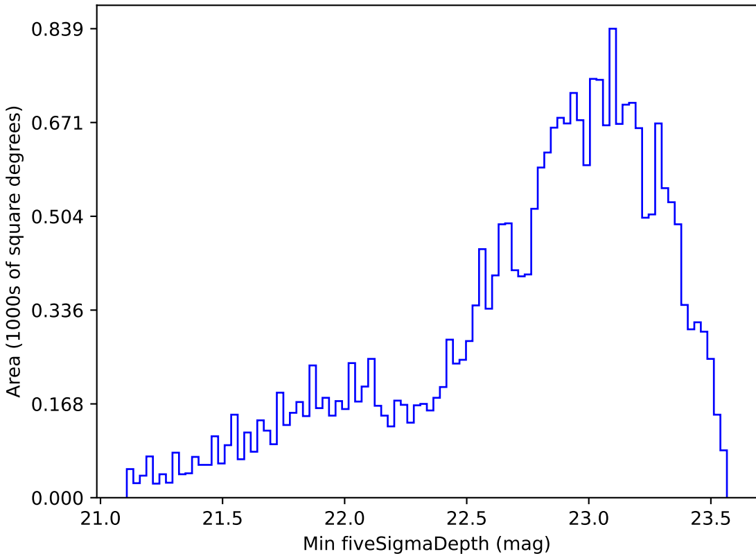
too_elab_r32_d3_griz_v3.4_10yrs Yr 1 i band: Min fiveSigmaDepth
