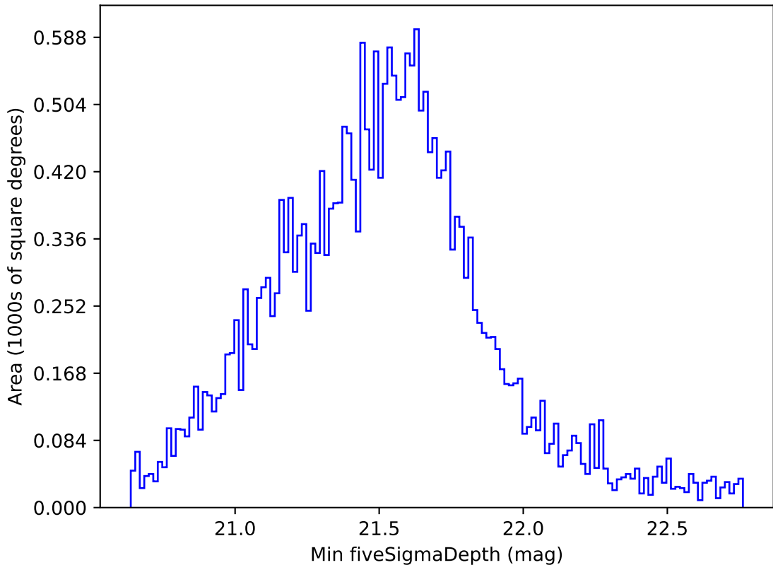
too_elab_r32_d3_griz_v3.4_10yrs Yr 1 all bands: Min fiveSigmaDepth
