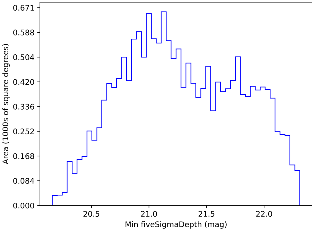
too_elab_r32_d3_griz_v3.4_10yrs WFD z band: Min fiveSigmaDepth
