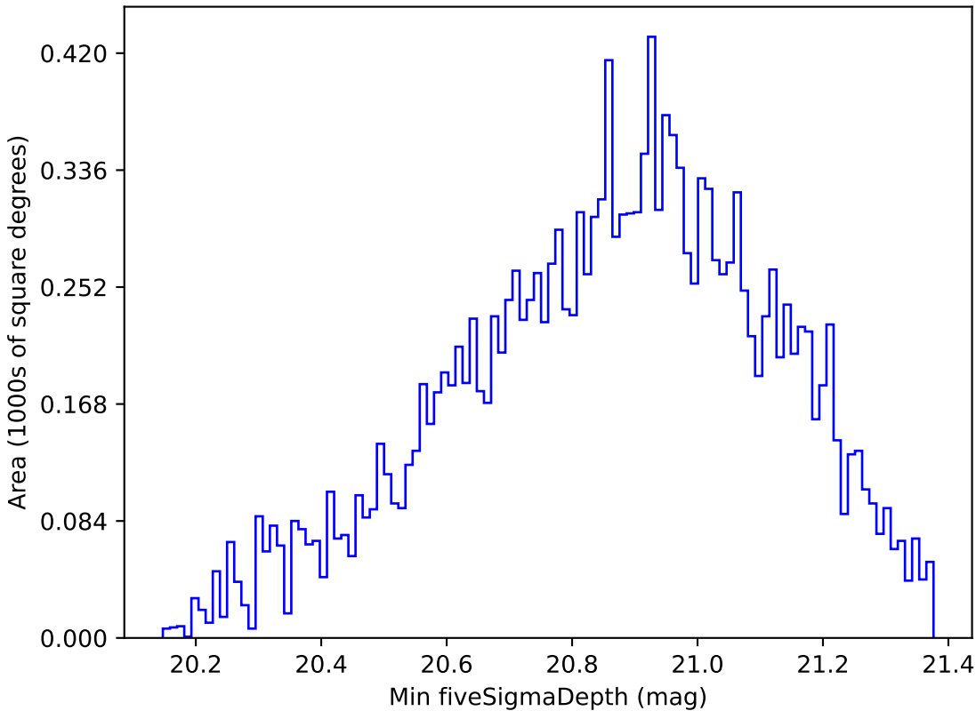
too_elab_r32_d3_griz_v3.4_10yrs WFD y band: Min fiveSigmaDepth
