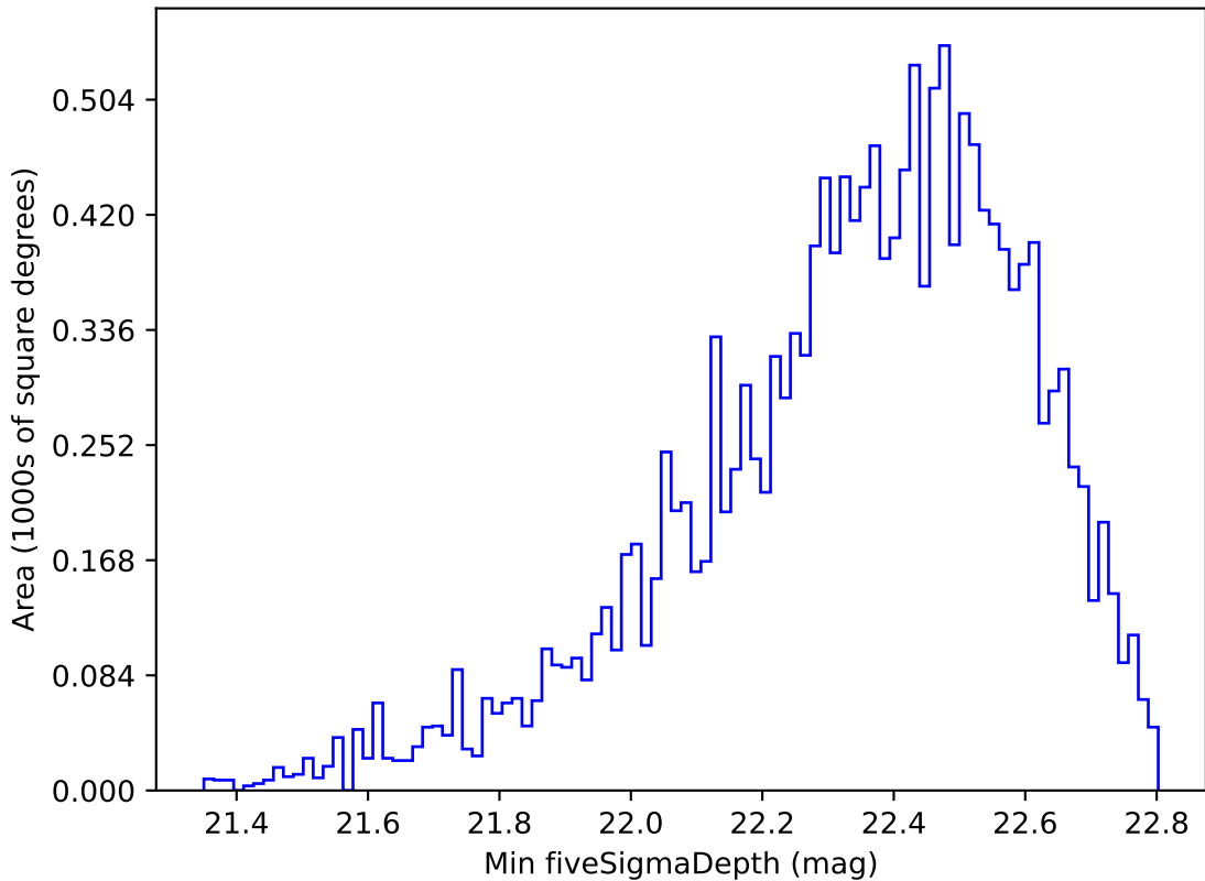
too_elab_r32_d3_griz_v3.4_10yrs WFD u band: Min fiveSigmaDepth
