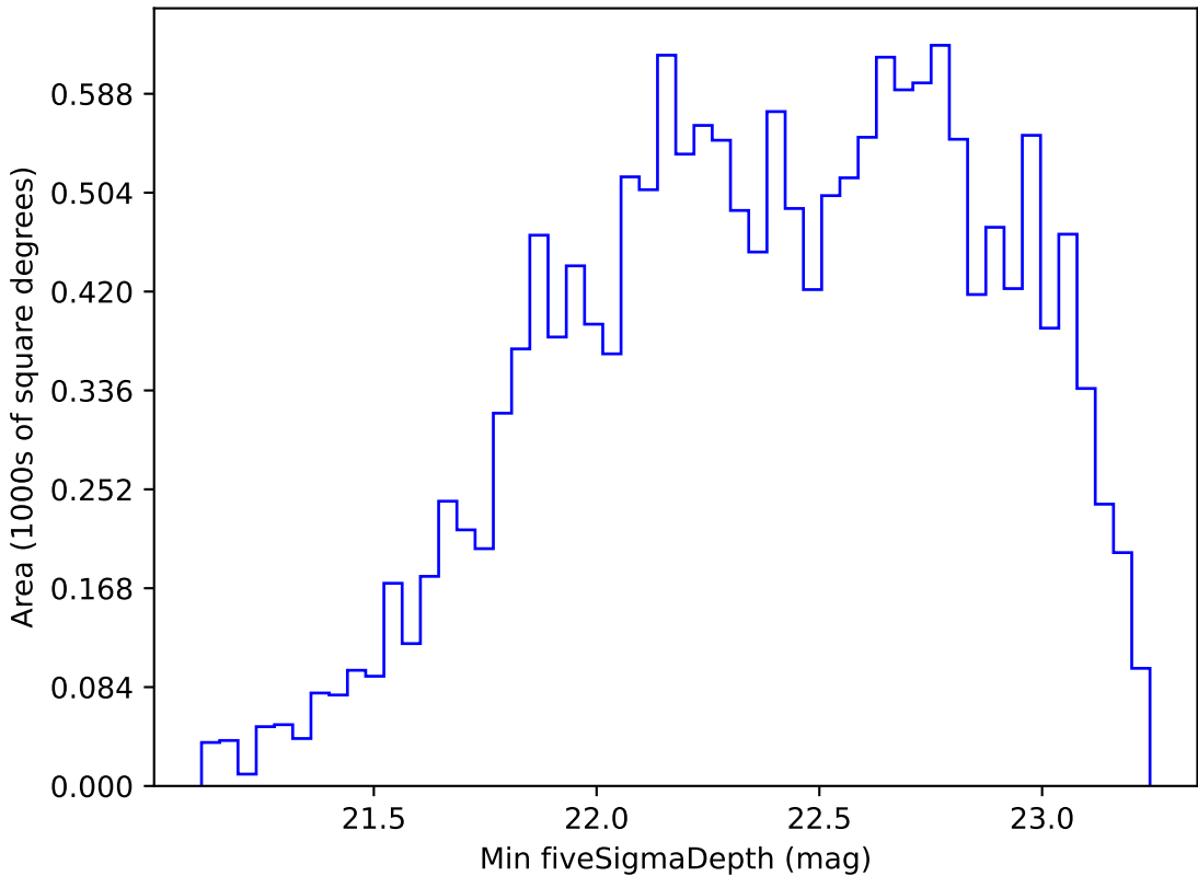
too_elab_r32_d3_griz_v3.4_10yrs WFD r band: Min fiveSigmaDepth
