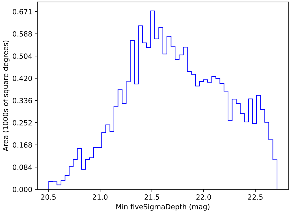
too_elab_r32_d3_griz_v3.4_10yrs WFD i band: Min fiveSigmaDepth
