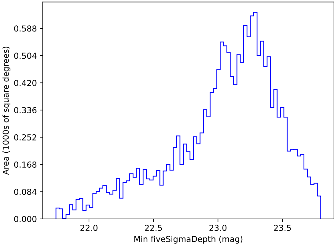
too_elab_r32_d3_griz_v3.4_10yrs WFD g band: Min fiveSigmaDepth
