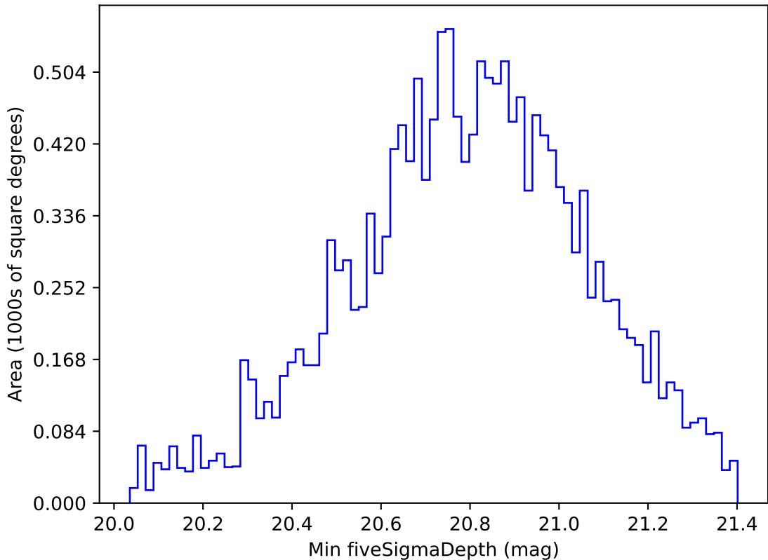
too_elab_r32_d3_griz_v3.4_10yrs WFD all bands: Min fiveSigmaDepth
