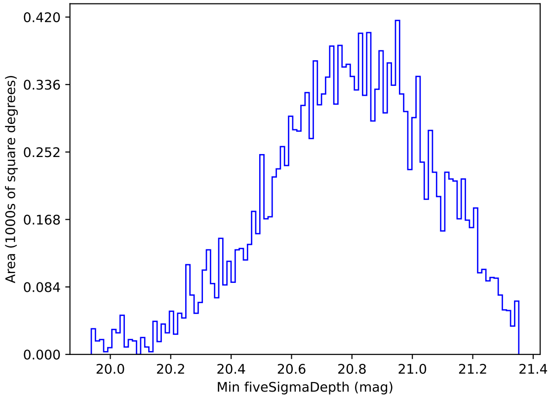
too_elab_r32_d3_griz_v3.4_10yrs WFD all bands: Min fiveSigmaDepth
