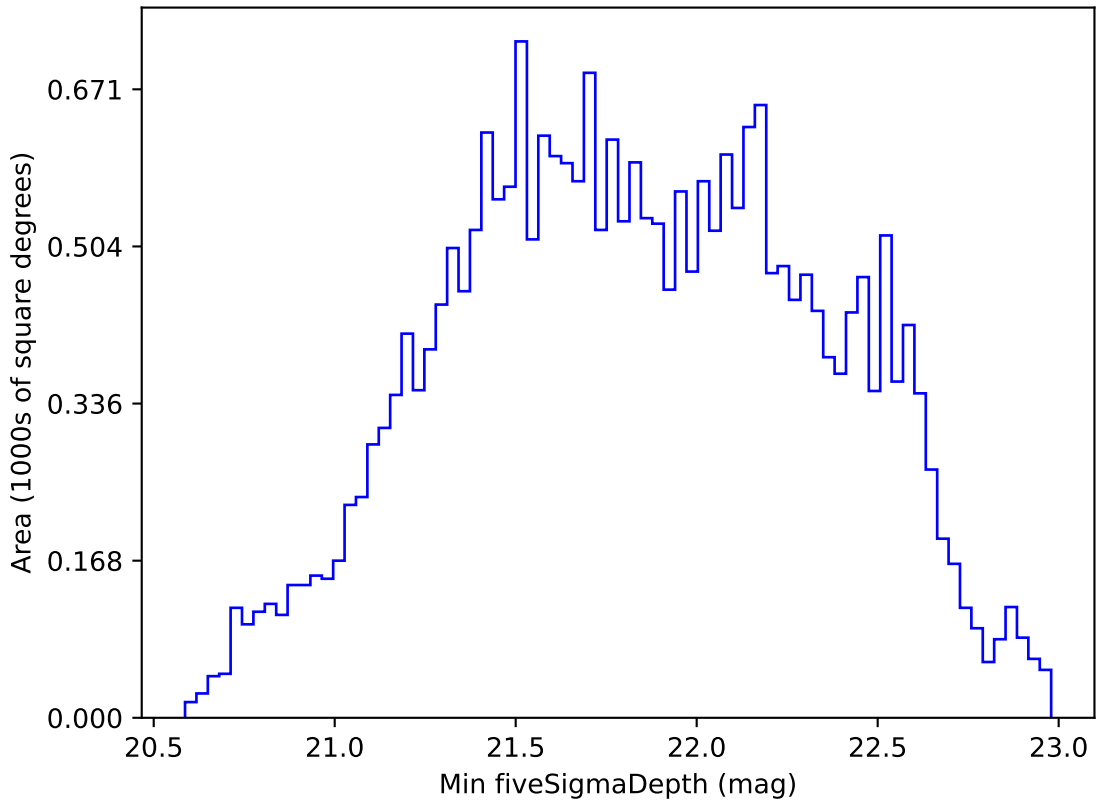
too_elab_r32_d3_griz_v3.4_10yrs All sky i band: Min fiveSigmaDepth
