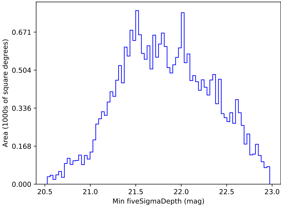
too_elab_r32_d3_griz_v3.4_10yrs All sky i band: Min fiveSigmaDepth
