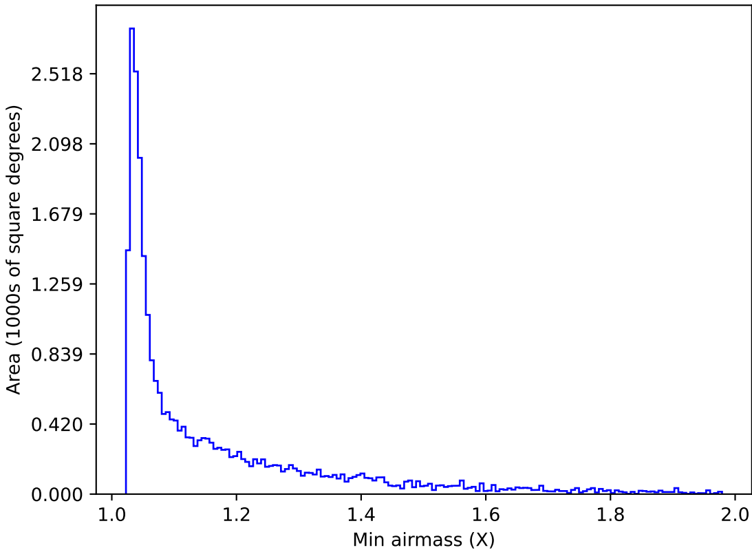
too_elab_r32_d3_griz_v3.4_10yrs Yr 1 i band: Min airmass
