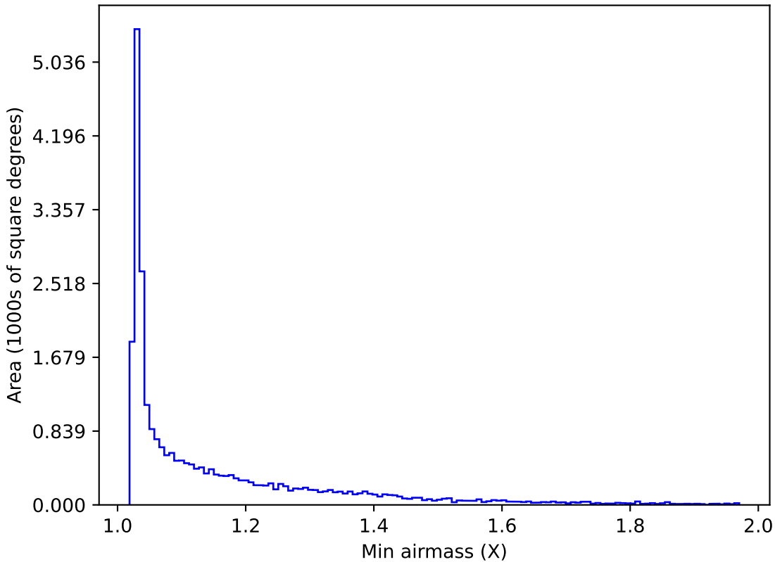
too_elab_r32_d3_griz_v3.4_10yrs Yr 1 all bands: Min airmass
