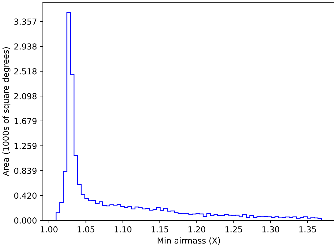
too_elab_r32_d3_griz_v3.4_10yrs WFD z band: Min airmass
