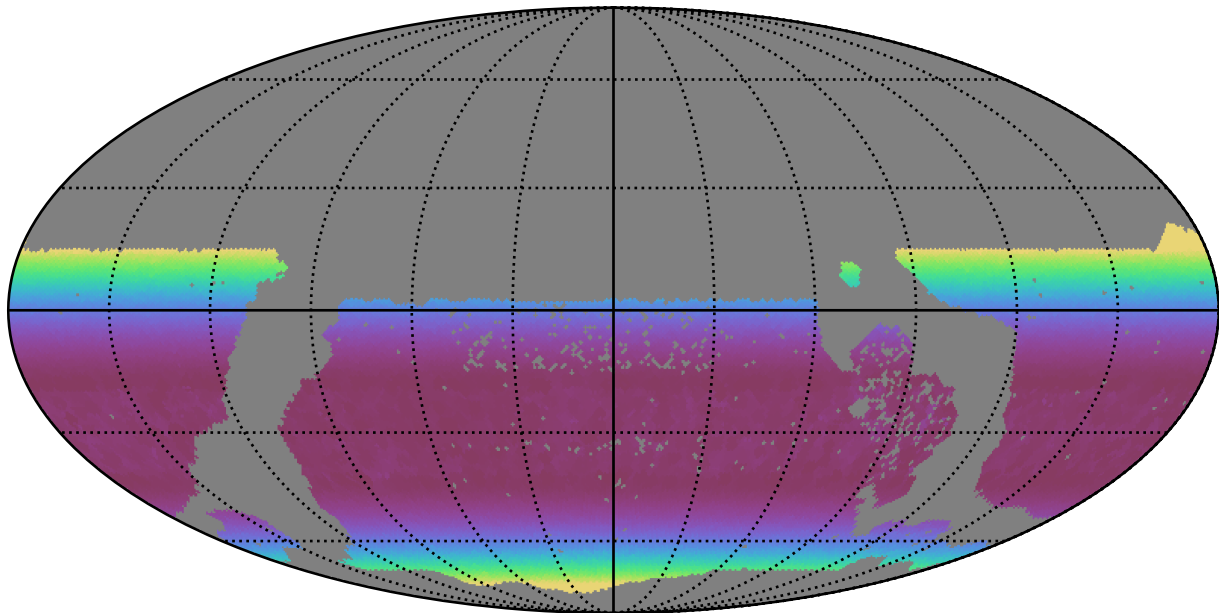
too_elab_r32_d3_griz_v3.4_10yrs WFD y band: Min airmass
