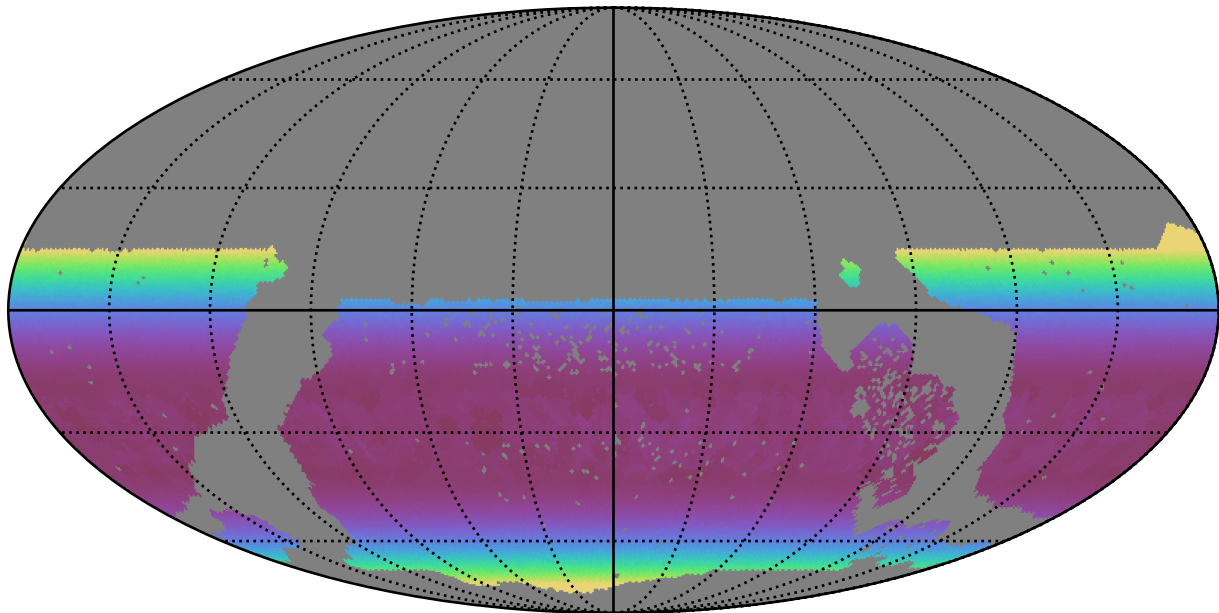
too_elab_r32_d3_griz_v3.4_10yrs WFD r band: Min airmass
