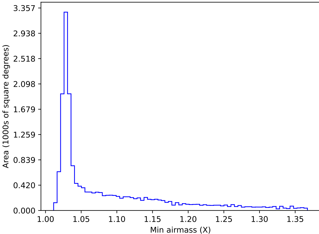
too_elab_r32_d3_griz_v3.4_10yrs WFD i band: Min airmass
