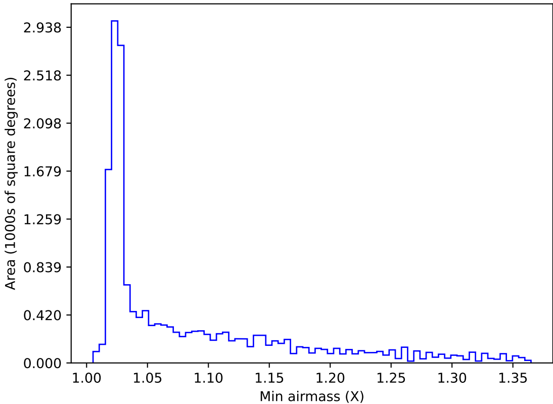
too_elab_r32_d3_griz_v3.4_10yrs WFD all bands: Min airmass
