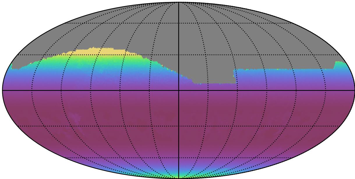
too_elab_r32_d3_griz_v3.4_10yrs All sky z band: Min airmass
