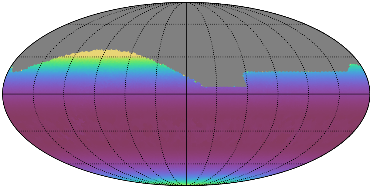
too_elab_r32_d3_griz_v3.4_10yrs All sky r band: Min airmass
