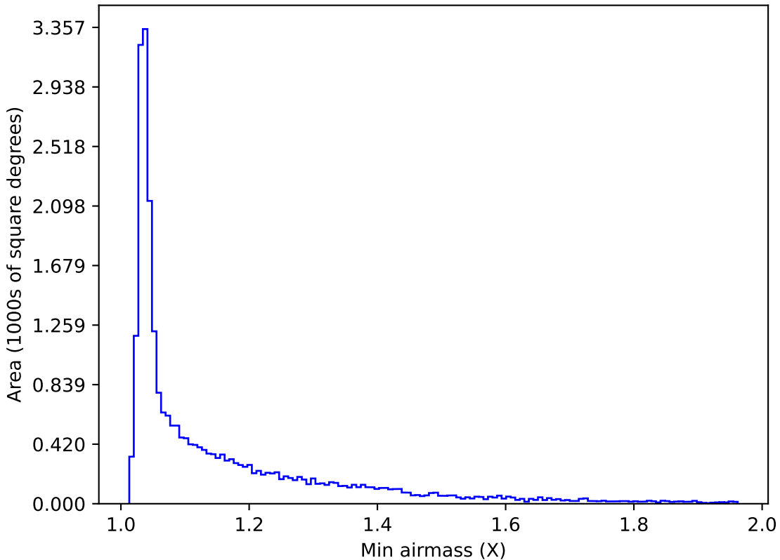
too_elab_r32_d3_griz_v3.4_10yrs All sky g band: Min airmass
