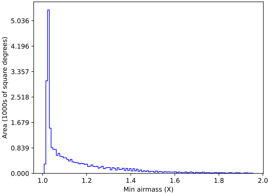
too_elab_r32_d3_griz_v3.4_10yrs All sky all bands: Min airmass
