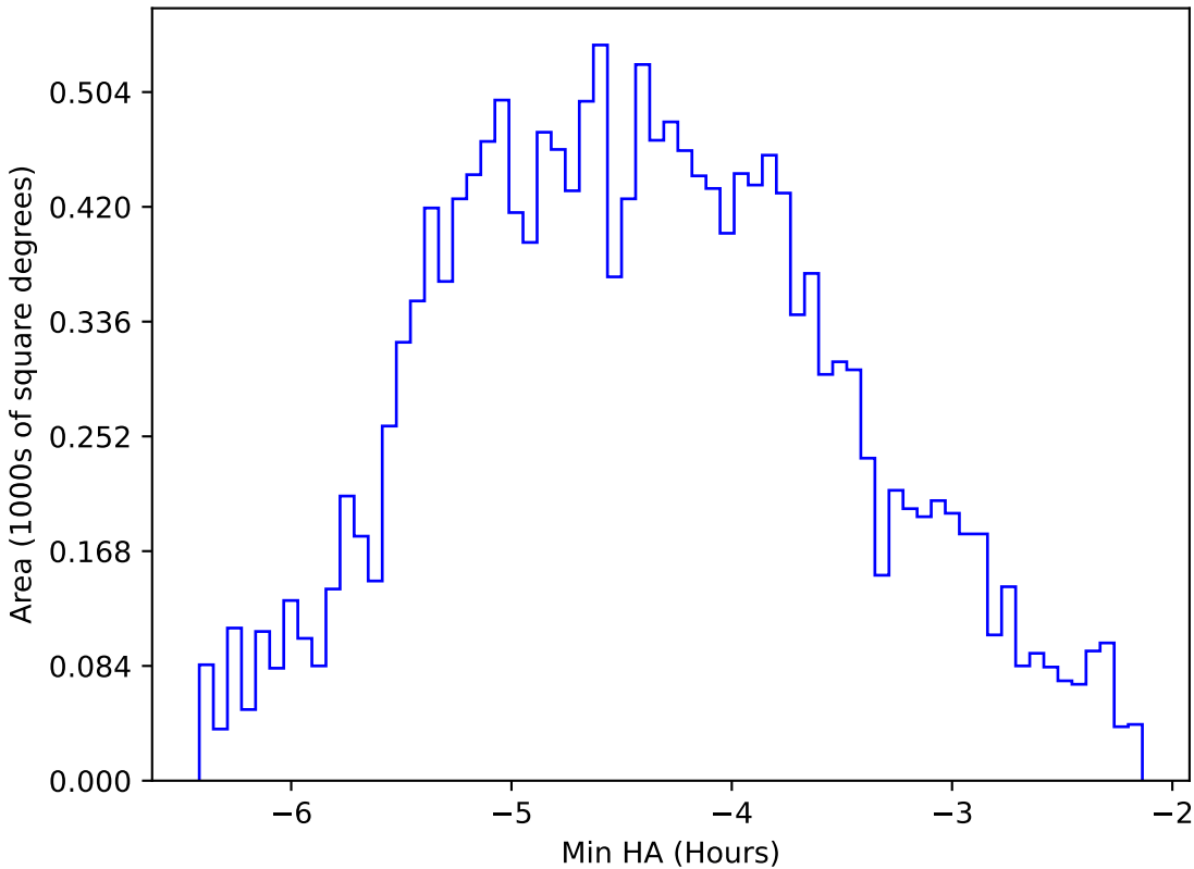
too_elab_r32_d3_griz_v3.4_10yrs WFD z band: Min HA
