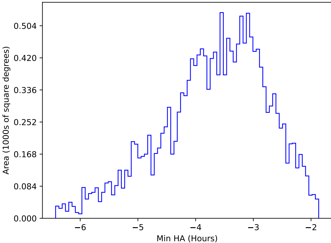
too_elab_r32_d3_griz_v3.4_10yrs WFD y band: Min HA
