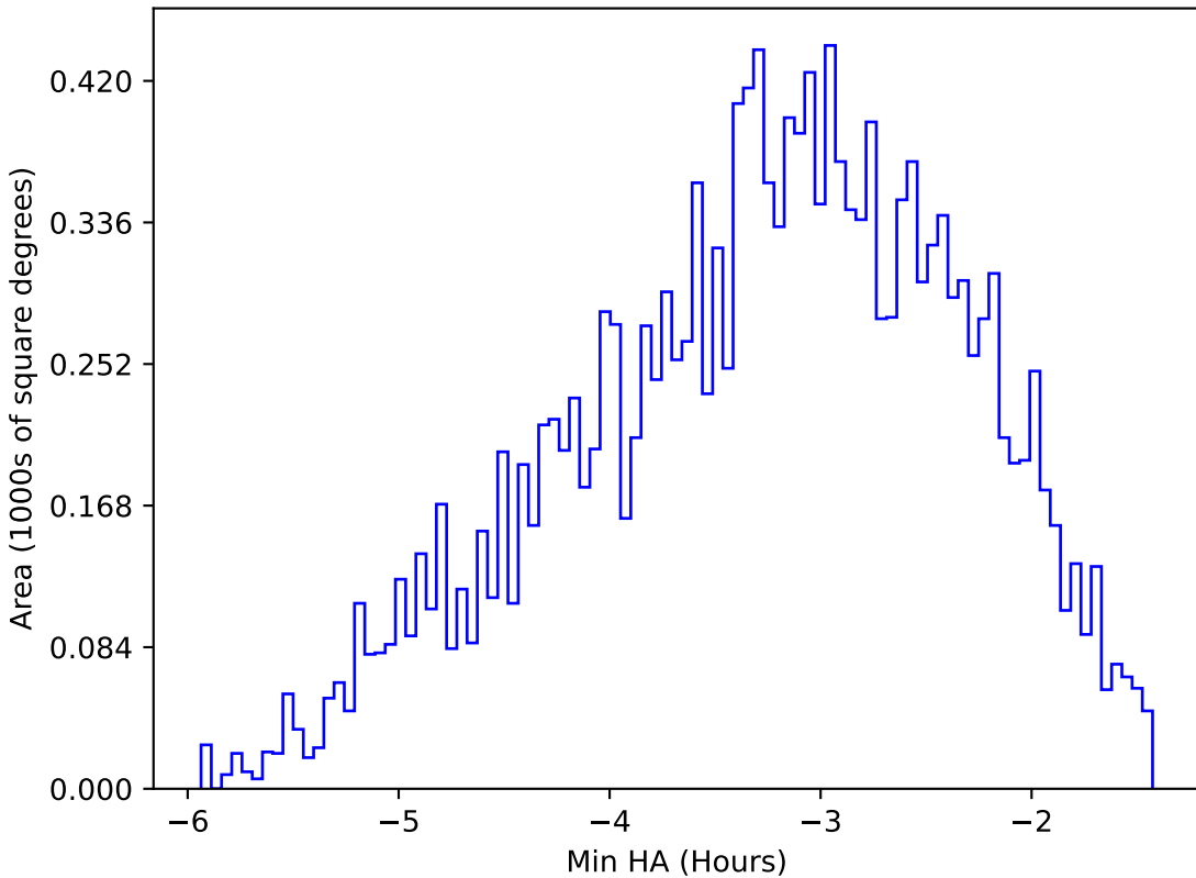
too_elab_r32_d3_griz_v3.4_10yrs WFD u band: Min HA
