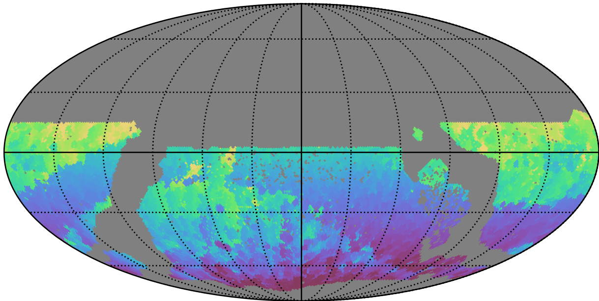
too_elab_r32_d3_griz_v3.4_10yrs WFD r band: Min HA
