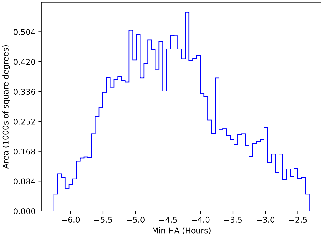
too_elab_r32_d3_griz_v3.4_10yrs WFD r band: Min HA
