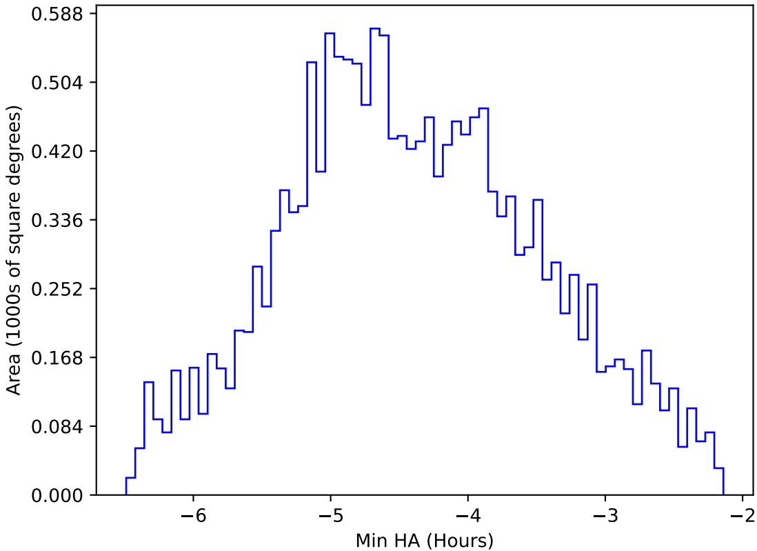
too_elab_r32_d3_griz_v3.4_10yrs WFD i band: Min HA
