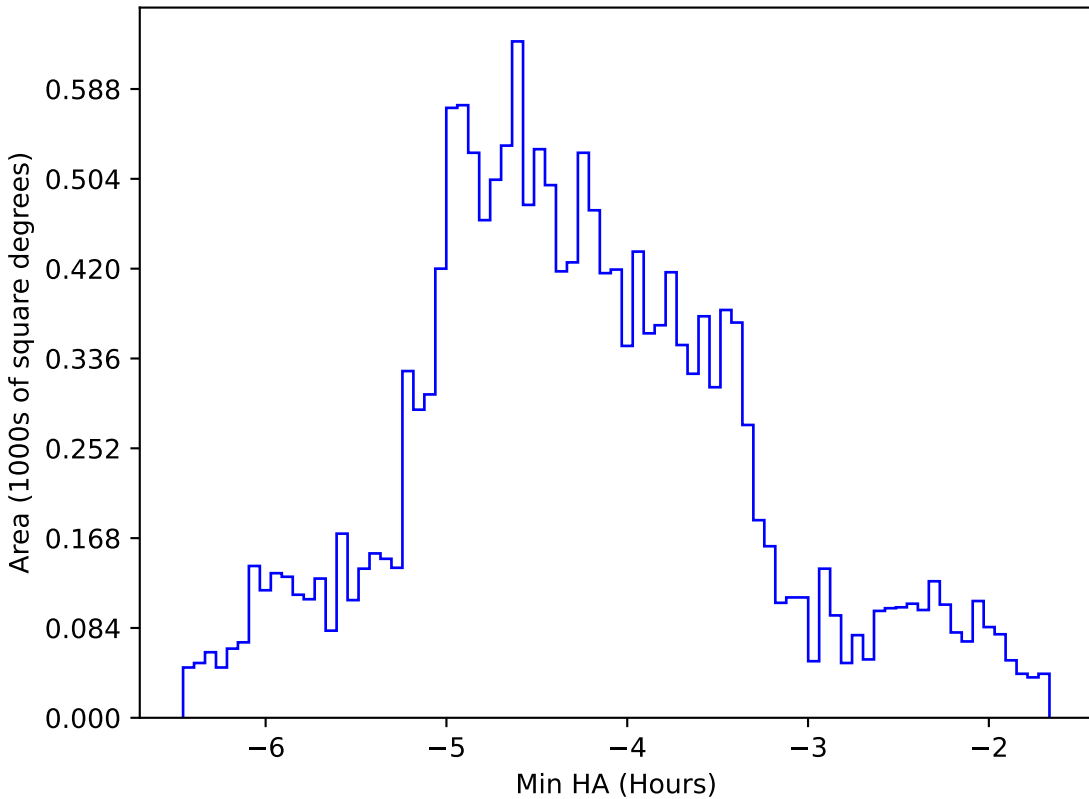
too_elab_r32_d3_griz_v3.4_10yrs WFD g band: Min HA
