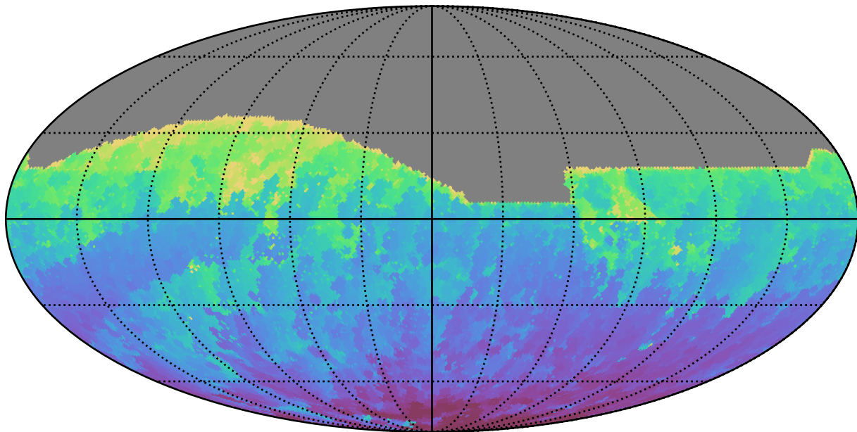
too_elab_r32_d3_griz_v3.4_10yrs All sky z band: Min HA
