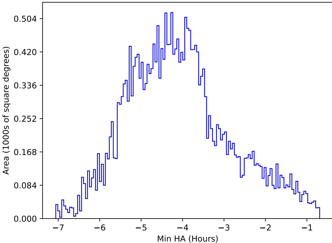
too_elab_r32_d3_griz_v3.4_10yrs All sky z band: Min HA
