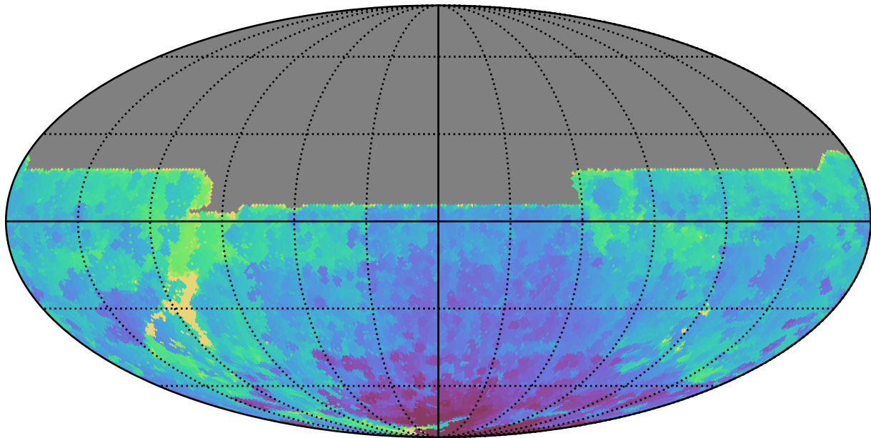
too_elab_r32_d3_griz_v3.4_10yrs All sky y band: Min HA
