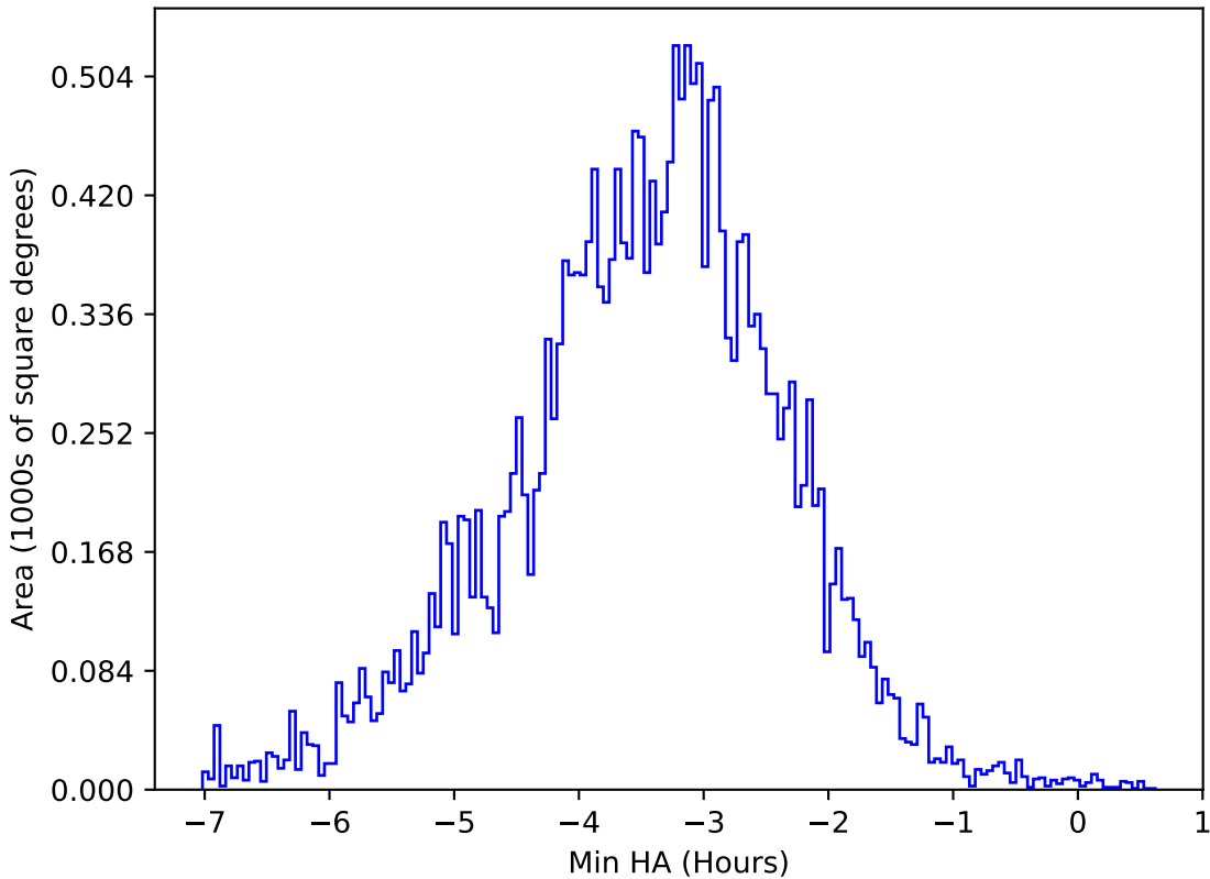
too_elab_r32_d3_griz_v3.4_10yrs All sky y band: Min HA
