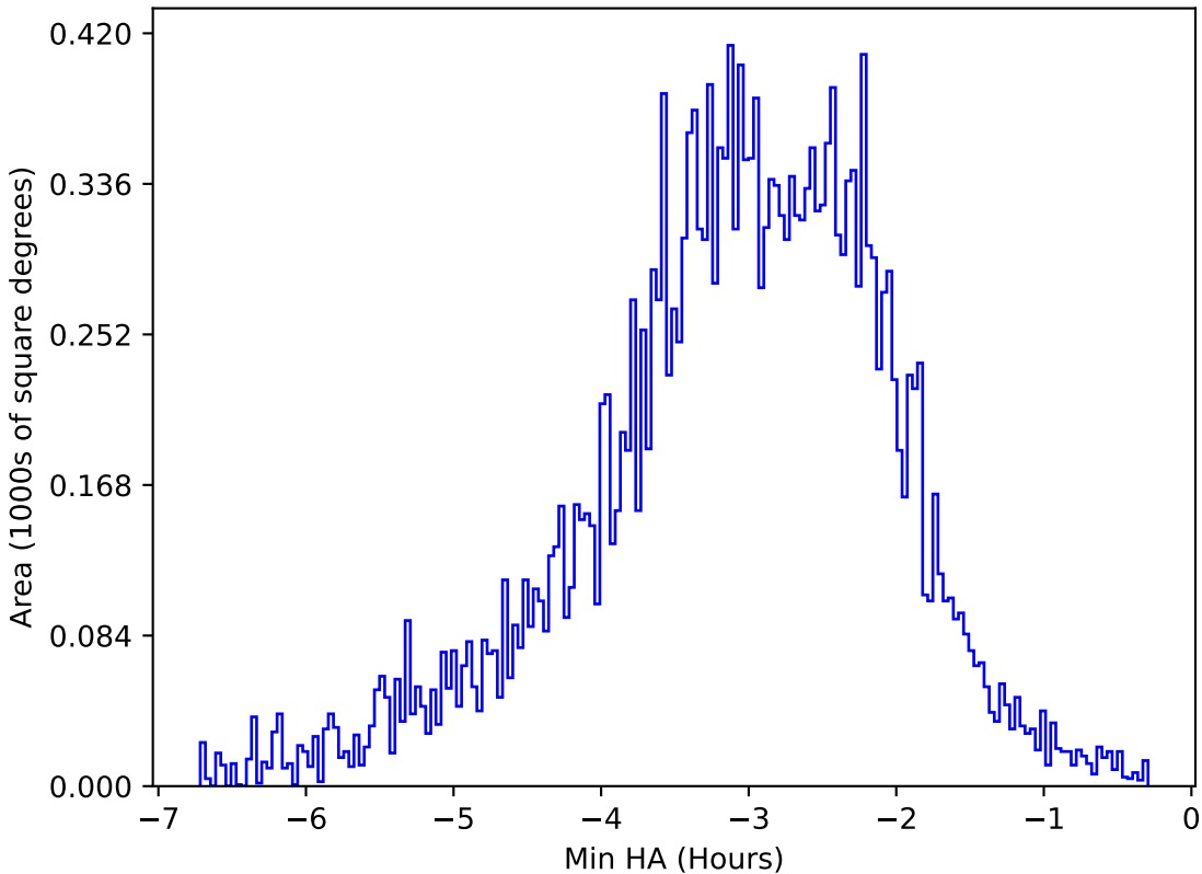
too_elab_r32_d3_griz_v3.4_10yrs All sky u band: Min HA
