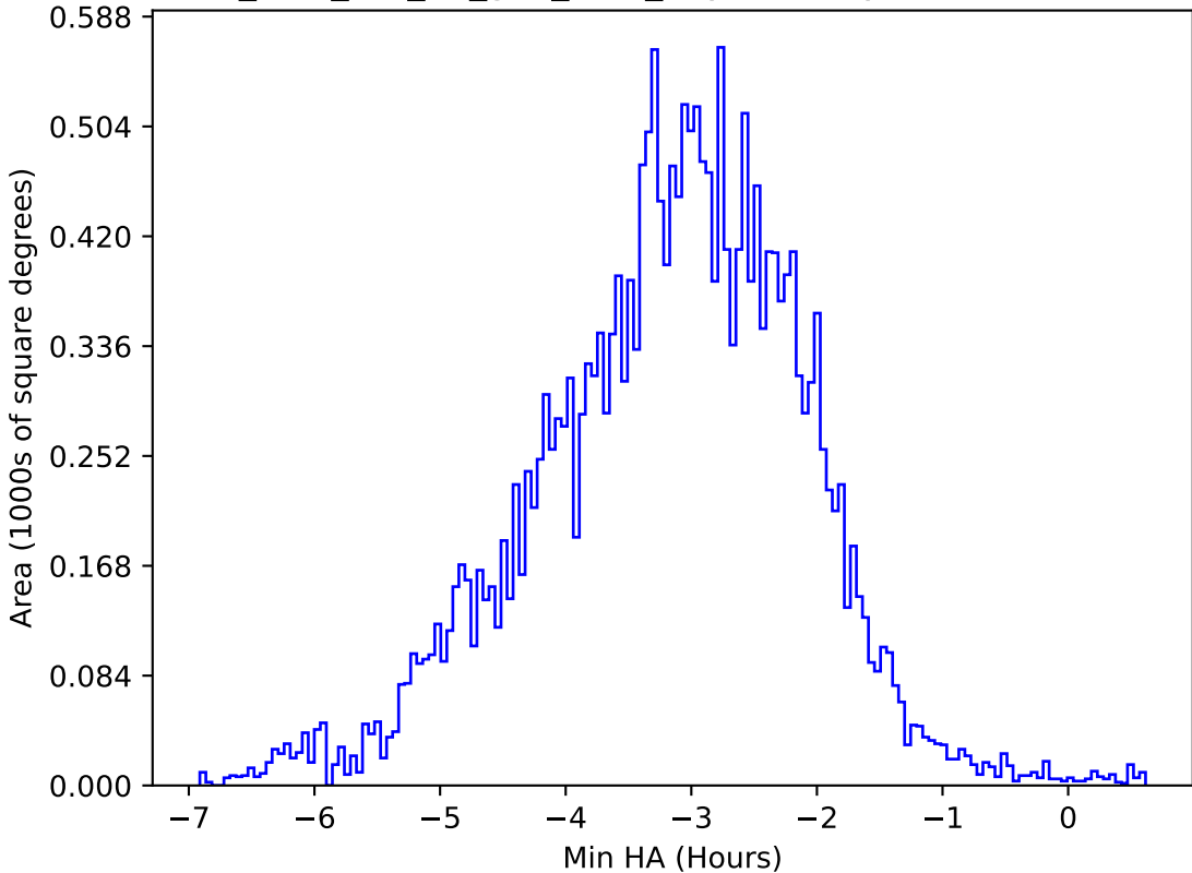
too_elab_r32_d3_griz_v3.4_10yrs All sky u band: Min HA
