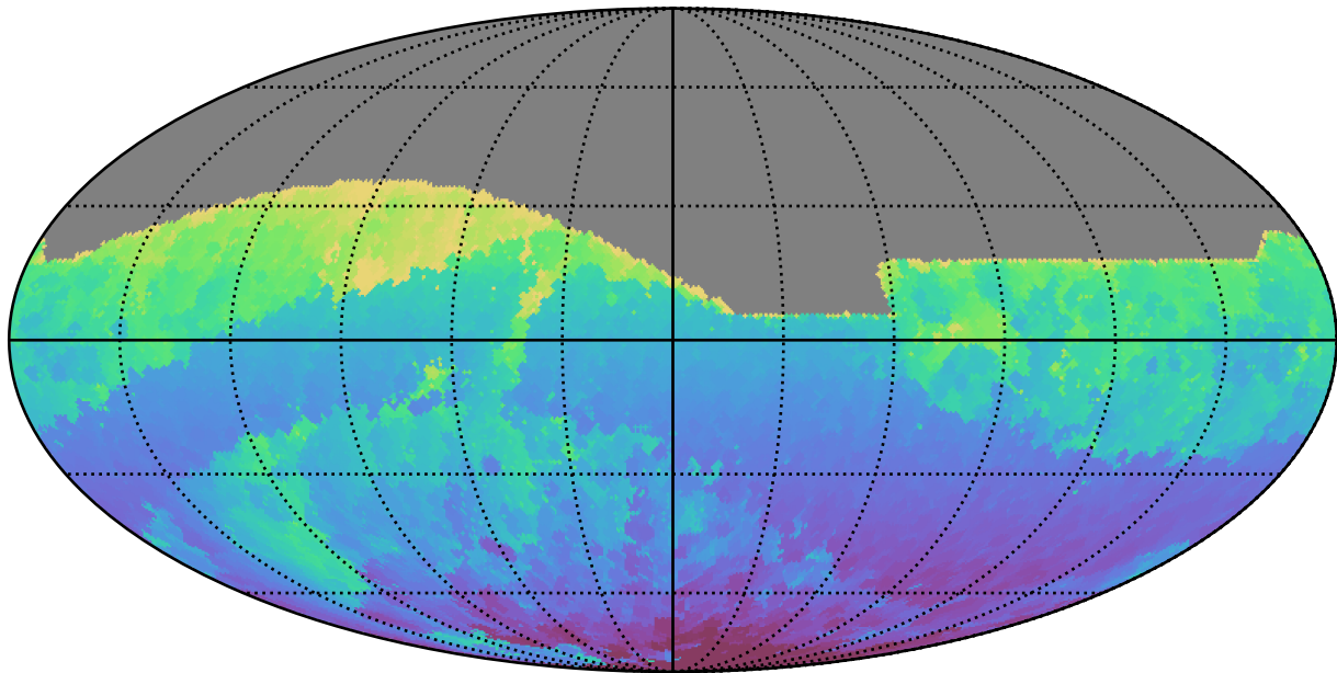
too_elab_r32_d3_griz_v3.4_10yrs All sky r band: Min HA
