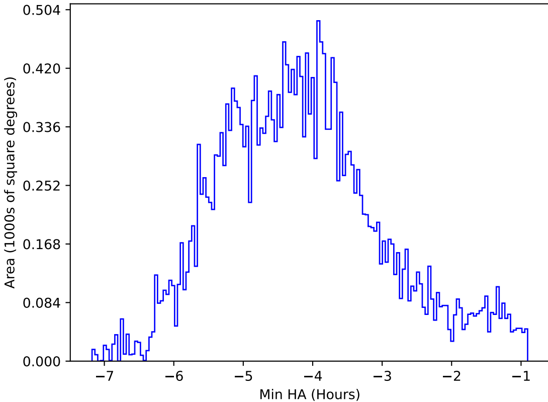
too_elab_r32_d3_griz_v3.4_10yrs All sky r band: Min HA
