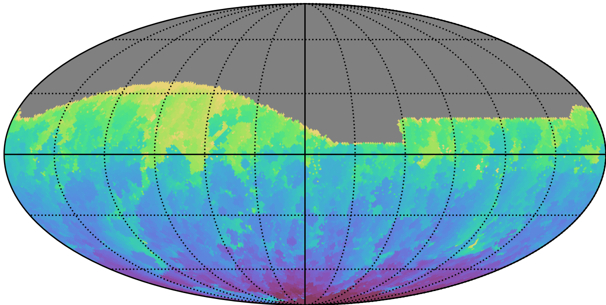
too_elab_r32_d3_griz_v3.4_10yrs All sky g band: Min HA
