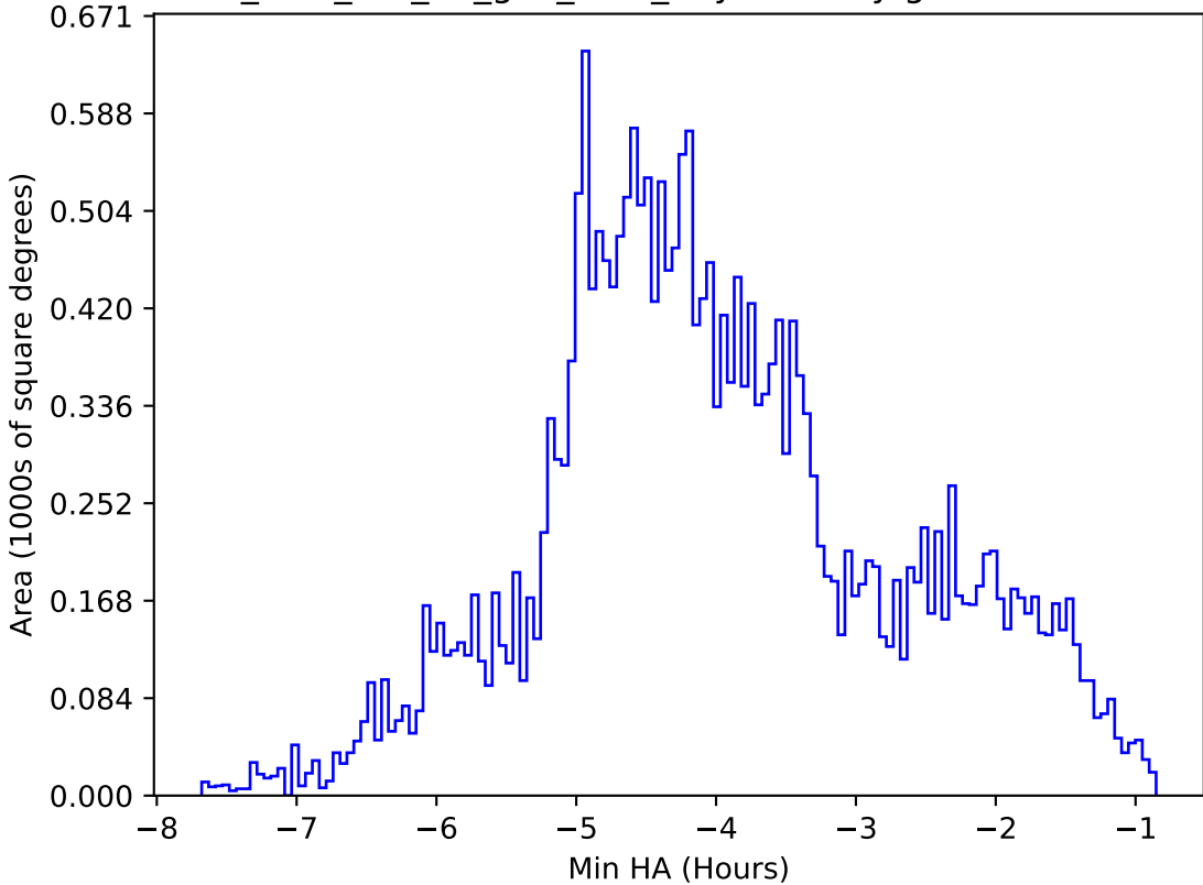
too_elab_r32_d3_griz_v3.4_10yrs All sky g band: Min HA
