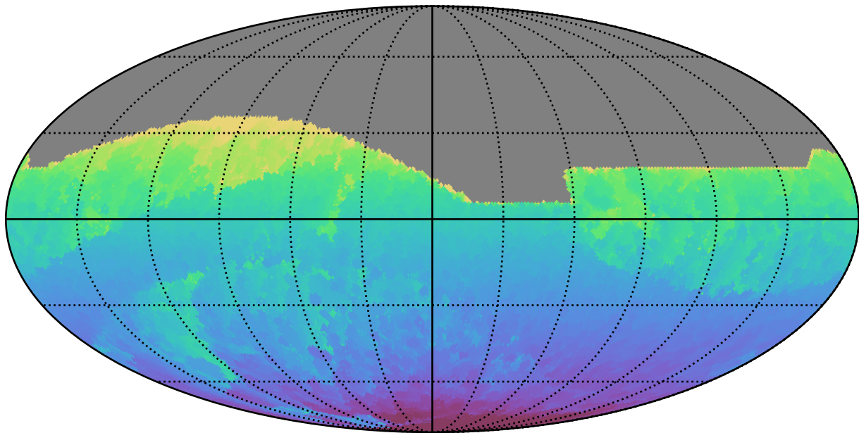
too_elab_r32_d3_griz_v3.4_10yrs All sky all bands: Min HA
