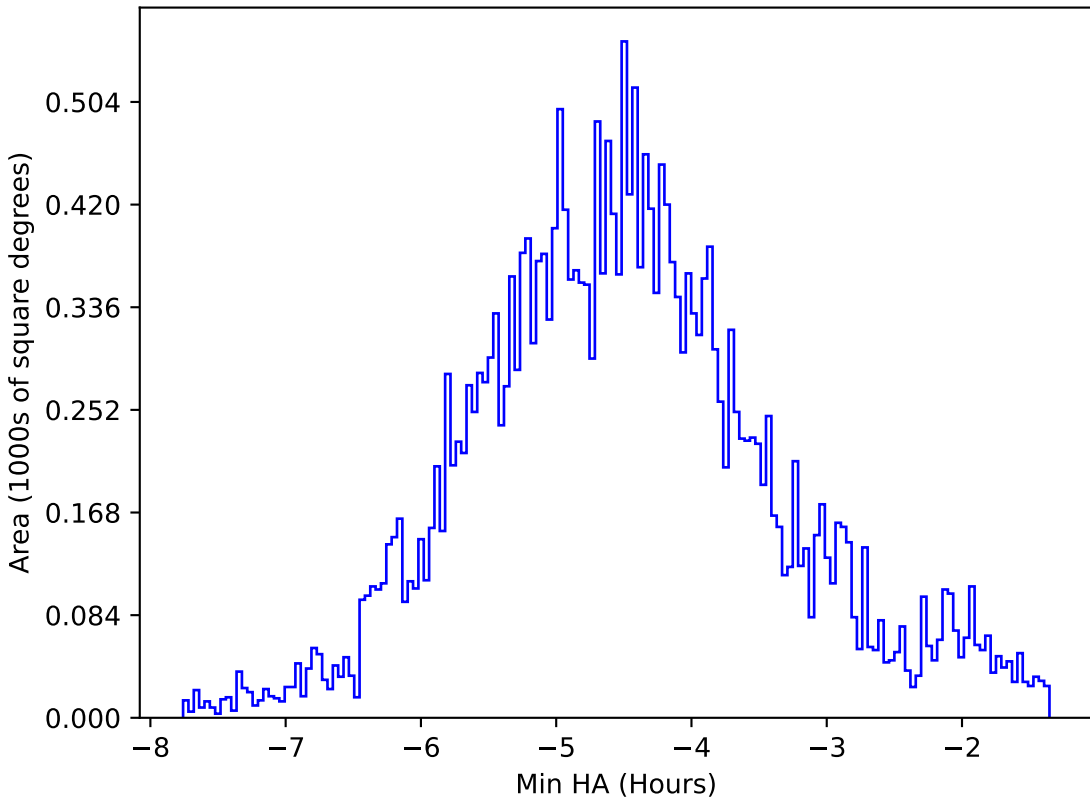
too_elab_r32_d3_griz_v3.4_10yrs All sky all bands: Min HA
