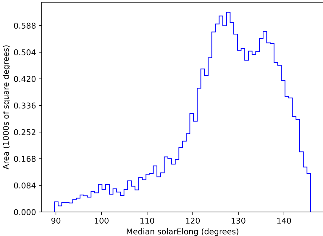
too_elab_r32_d3_griz_v3.4_10yrs WFD z band: Median solarElong
